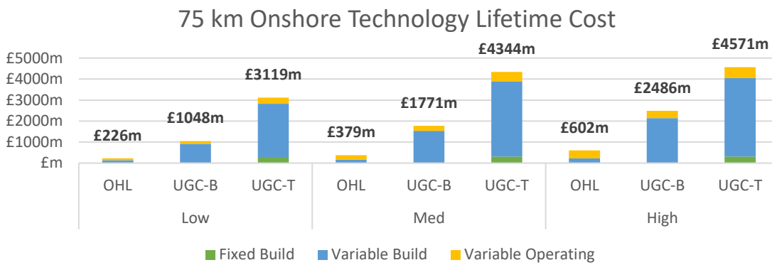
Figure 4.5: Onshore Technologies – 75 km Comparison
