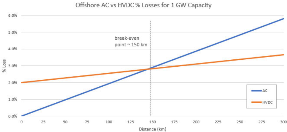
Figure I.1: Submarine AC versus HVDC Losses
