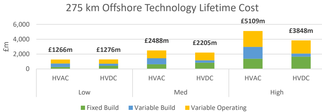
Figure 4.10: Offshore Technologies – 275 km Comparison
