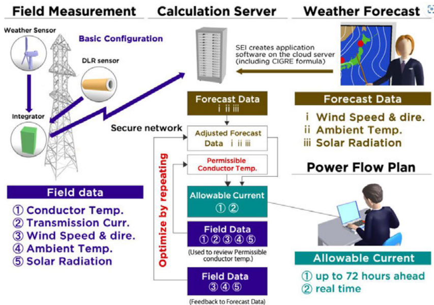
Figure D.28: Typical DLR diagram
