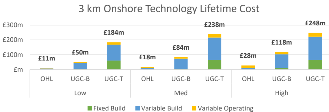
Figure 4.3: Onshore Technologies – 3 km Comparison
