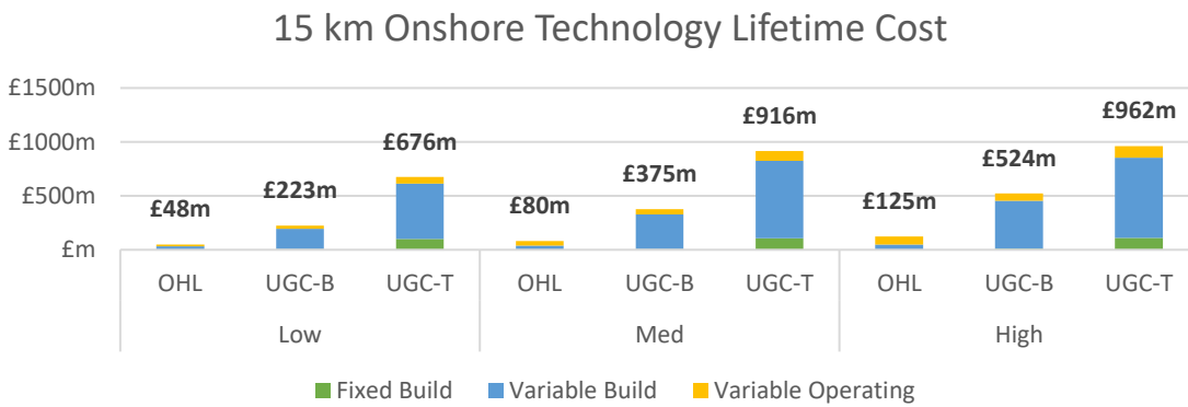
Figure 4.4: Onshore Technologies – 15 km Comparison
