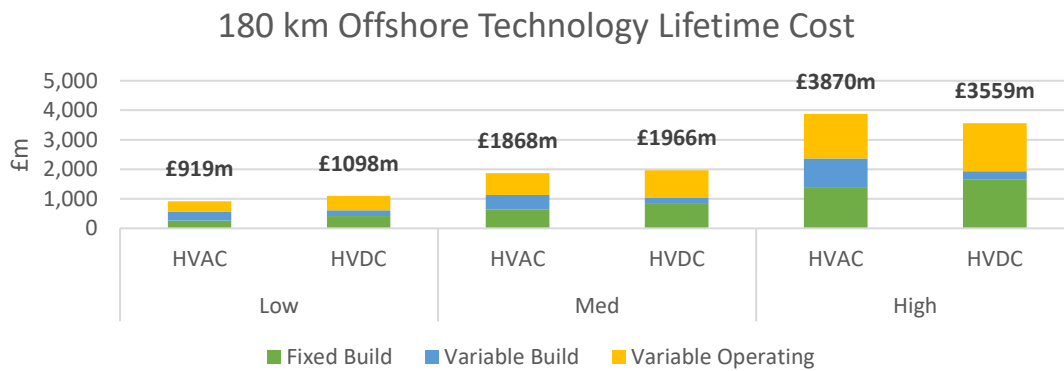
Figure 4.9: Offshore Technologies – 180 km Comparison
